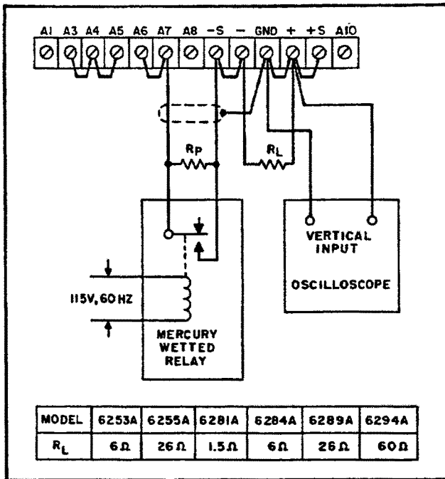
Figure 5-10. Constant Voltage Programming Speed, Test Setup
