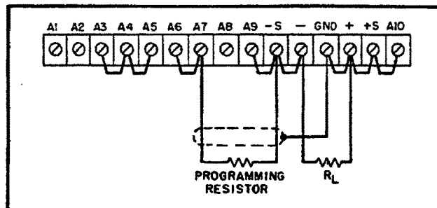
Figure 3-3. Remote Resistance Programming (Constant Voltage)
