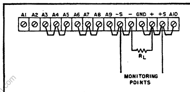
Figure 3-2. Normal Strapping Pattern
